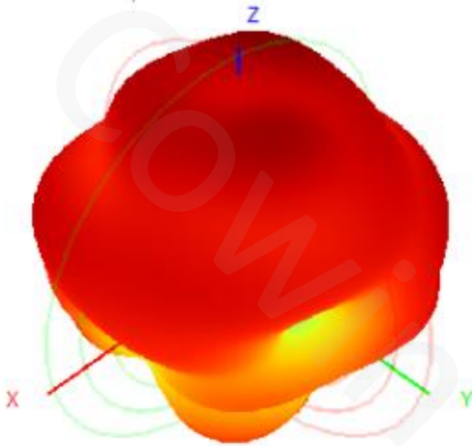
2500.0MHz H+V, Eff: 61.7%
