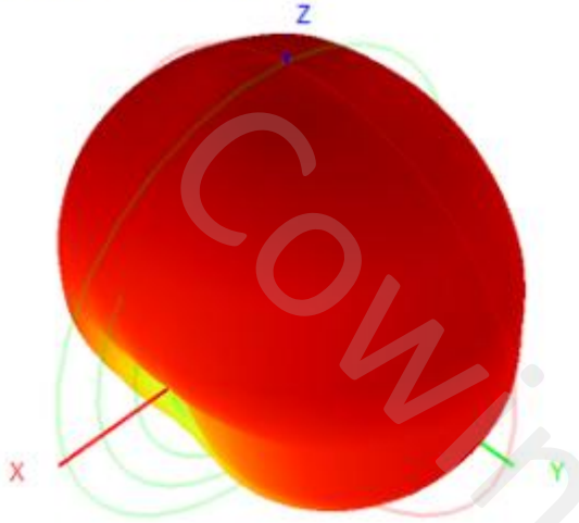
750.0MHz Total, Eff: 85.4%
